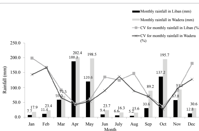
Figure 3: Monthly rainfall and coefficient of variation in Liben and Wadera districts of south Ethiopia.
