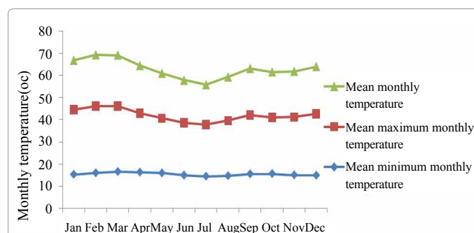
Figure 5: Monthly mean maximum and minimum temperature in Liben district (1985-2014) of South Ethiopia.
