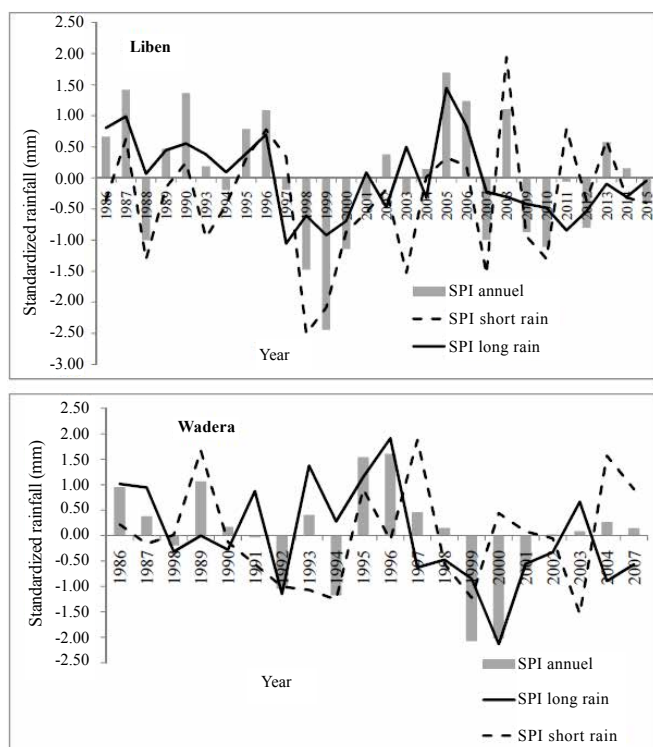
Figure 2: Standardized precipitation index for annual, long and short rainy season in Liben and Wadera districts of south Ethiopia.
