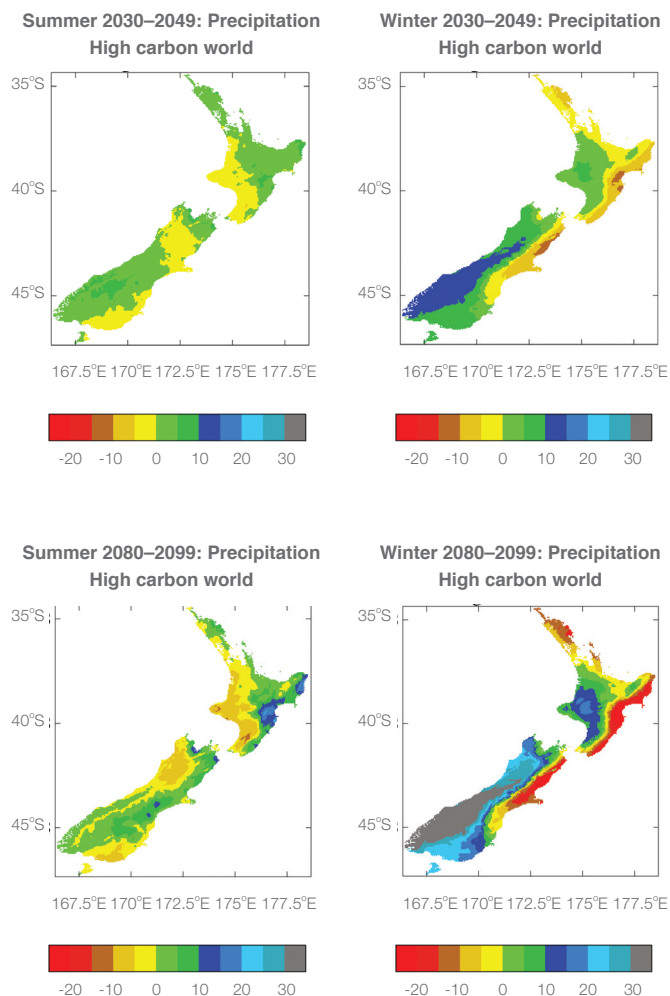
Figure 5b. Projected New Zealand seasonal precipitation change (in %) from 1980-1999 to 2030-2049 (upper panels), and to 2080-2099 (lower panels), for the high carbon world as averaged over the downscaled patterns from 12 global models. Summer and winter seasons are shown.
