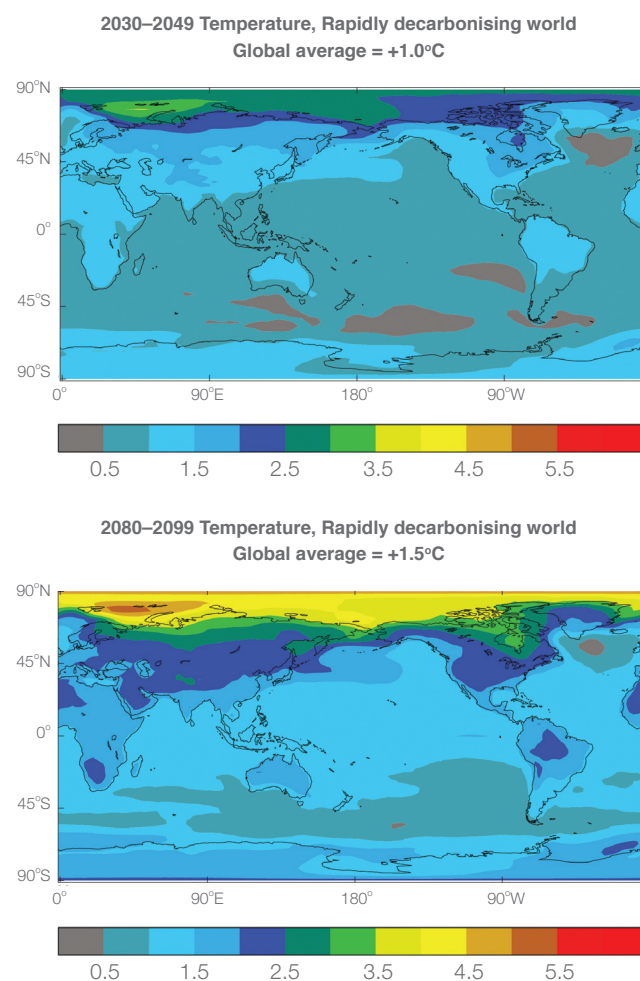
Figure 3. Global temperature change (in °C) from 1980–1999 to 2030–2049 (upper panel) and to 2080–2099 (lower panel) for the rapidly decarbonising world, as averaged over 12 global models. The global-average change is indicated in the figure heading.
