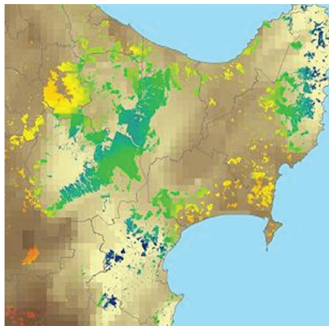
Figure 3. East Cape - projected summer rainfall changes in planted forests in 2040 under the high carbon world scenario (dark blue = +6%, orange = -6%).
