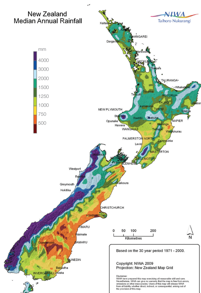
Figure 4. New Zealand median annual rainfall (mm).
