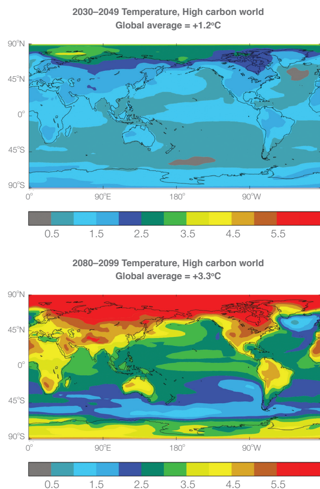
Figure 2. Global temperature change (in °C) from 1980–1999 to 2030–2049 (upper panel) and to 2080–2099 (lower panel) for the high carbon world, as averaged over 12 global models. The global-average change is indicated in the figure heading. For details on the selected models, see MfE (2008c).
