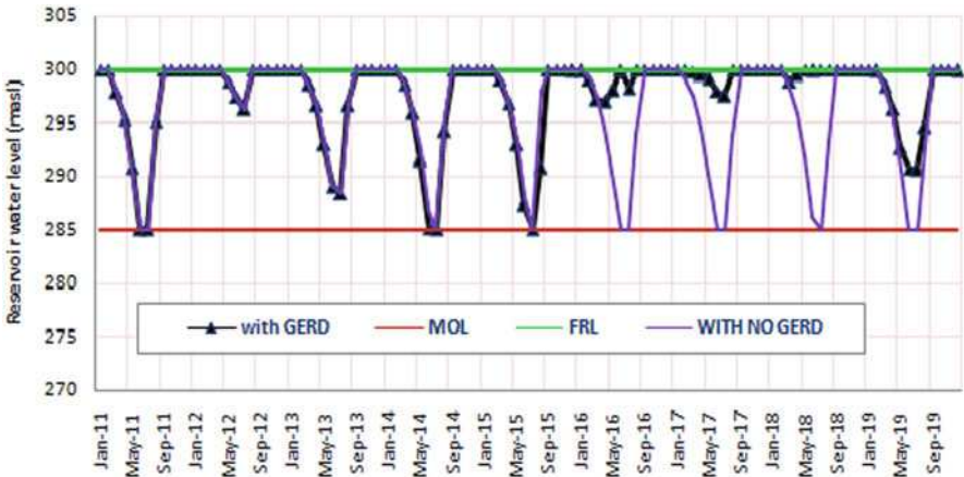
Fig. 27.13 Merowe reservoir pool level during impounding
