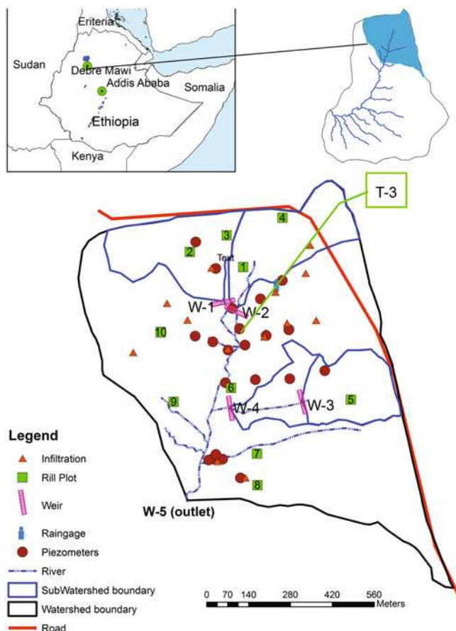
Fig. 9.1 Location, boundary, and drainage map of Debre Mawi with runoff and sediment concentration-monitoring sites (W), perched water table sampling (dark red circles) and infiltration test sites (red triangles), and agricultural field plots (numbers inside the green square boxes)
