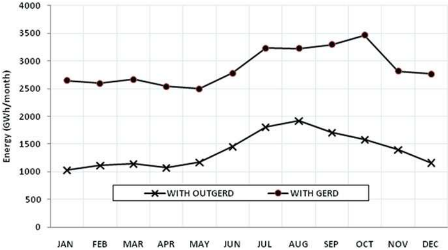
Fig. 27.17 Mean monthly Eastern Nile energy (GWh)
