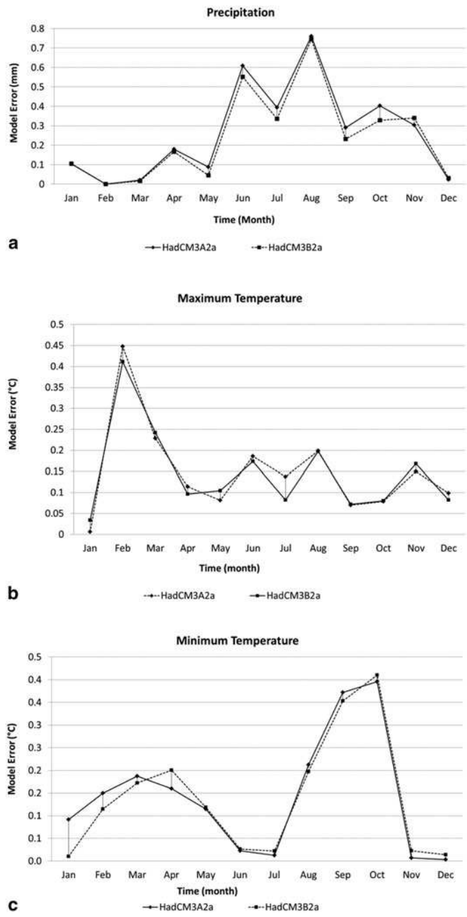
Fig. 19.9 Absolute model error of mean monthly precipitation (a), maximum temperature (b), and minimum temperature (c) (1961–1990)
