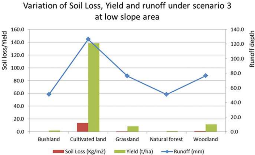
Fig. 10.11 Variation of soil loss, sediment yield, and runoff with land use/land cover under scenario 3 in low slope area as estimated by the model
