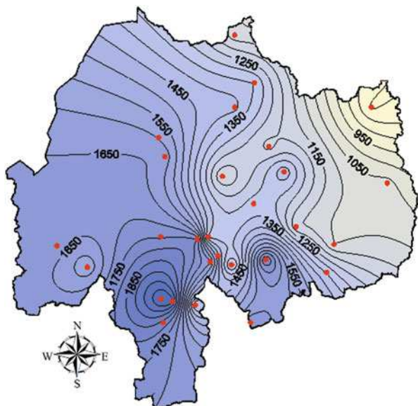
Fig. 2.8 Spatial variation of annual rainfall in the Blue Nile basin. (Abtew et al. 2009)
