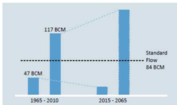
Fig. 25.3 Oscillations in Nile flow. (Source: Blue Peace for the Nile, March 2013)
