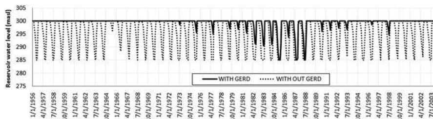
Fig. 27.16 Merowe water level during operation
