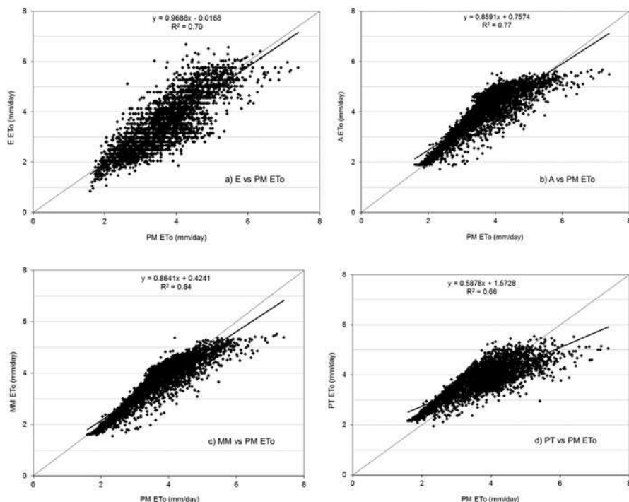
Fig. 16.4 Scatter plots of different methods with PM ETo at Debre Markos station
