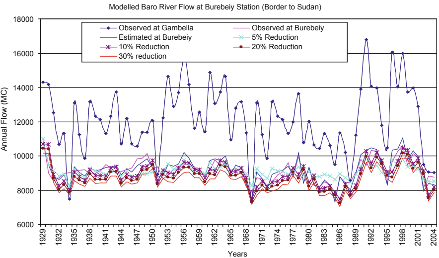
Fig. 18.6 Sensitivity outputs of Baro reach: Gambella–Burebeiy
