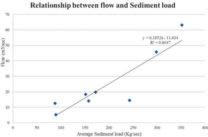
Fig. 10.19 Relationship of average measured sediment load variation with flow in Ruvu catchment
