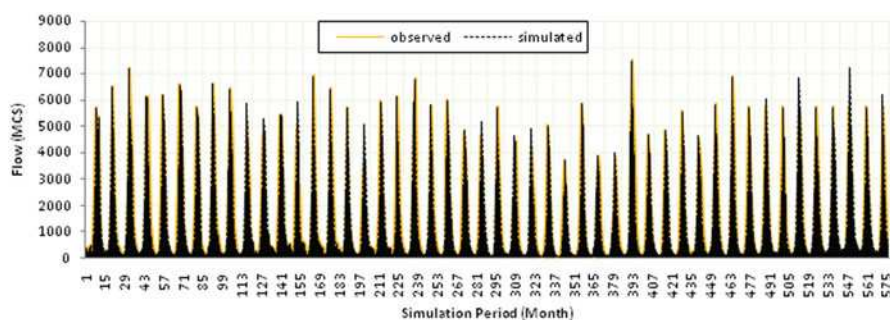
Fig. 27.2 Comparison of time series of simulated and input flow data at El Deim
