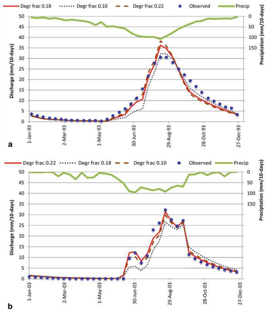
Fig. 8.3 a Observed ( closed spheres ) and predicted discharge ( solid line ) for the Blue Nile at El Diem at the Ethiopian Sudan border for three fractions of degraded hillsides for 1993, 10 % ( dotted line ), 18 % ( solid line ), and 22 % ( dashed line ). b Observed ( closed spheres ) and predicted discharge ( solid line ) for the Blue Nile at El Diem at the Ethiopian Sudan border for three fractions of degraded hillsides for 2003, 10 % ( dashed line ), 18 % ( dotted line ), and 22 % ( solid line )
