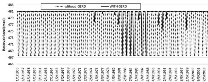
Fig. 27.14 Rosaries water level during operation of Grand Ethiopian Renaissance Dam Project (GERD)
