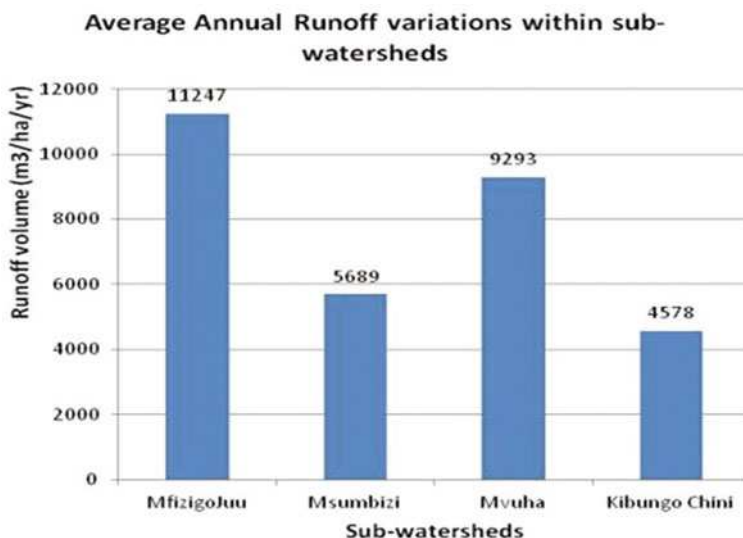
Fig. 10.8 Average annual runoff variations within the subwatersheds as estimated by the model
