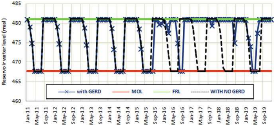
Fig. 27.11 Rosaries reservoir pool level during impounding
